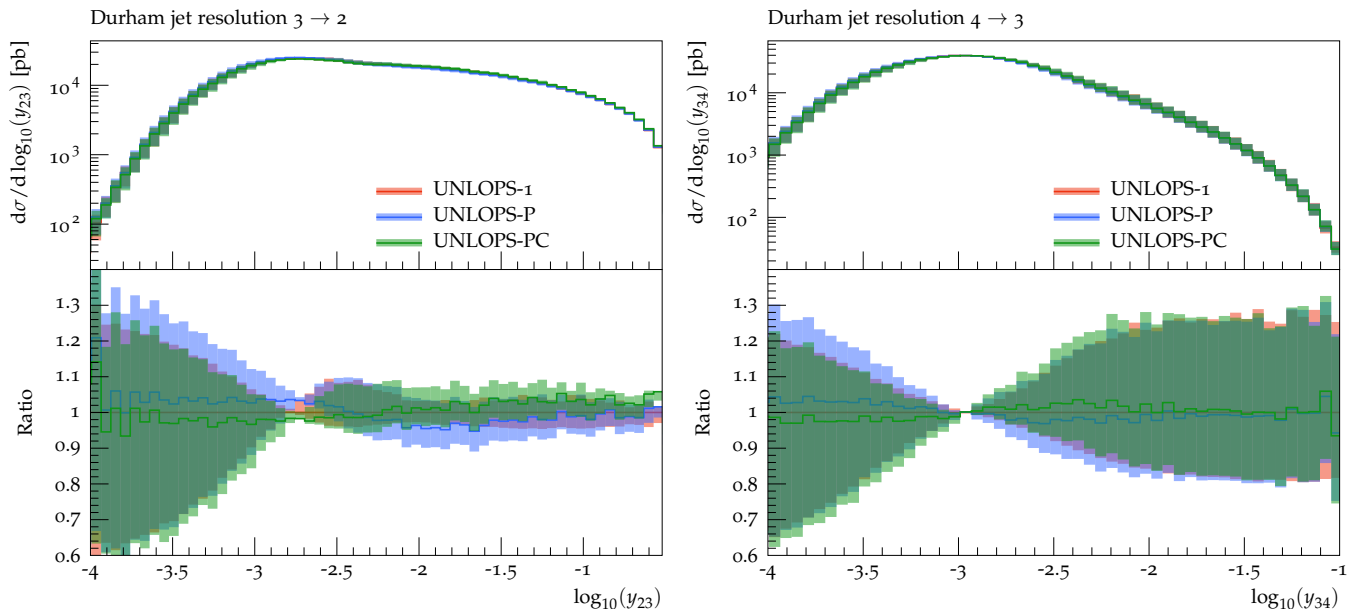
FIG. 1: Differential jet separation distributions y_{23} and y_{34} in e^+e^- \rightarrow jets at \sqrt{s} = M_Z . The left distribution is described at NLO accuracy at high scales, the right at LO accuracy for all jet separations.
