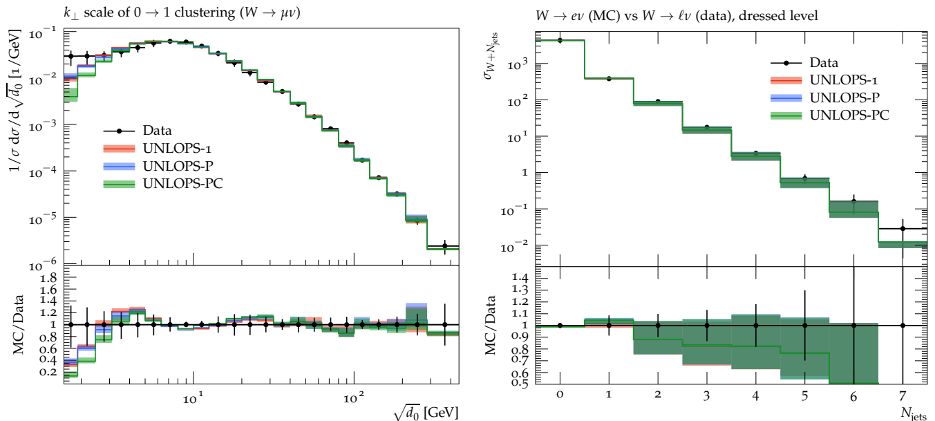
FIG. 3: W + \text{jets} production at proton proton collisions with \sqrt{s} = 7 TeV: k_{\perp} splitting scale of first jet [28] and exclusive jet multiplicity [29].
