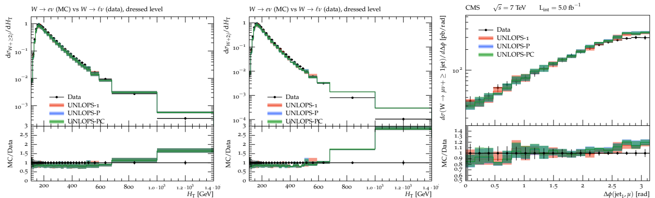
FIG. 4: W + \text{jets} production at proton proton collisions with \sqrt{s} = 7 TeV: Scalar sum of jet transverse momenta H_T for inclusive and exclusive 2 jet events [29] and azimuthal distance \Delta\phi between hardest jet and muon [32].
