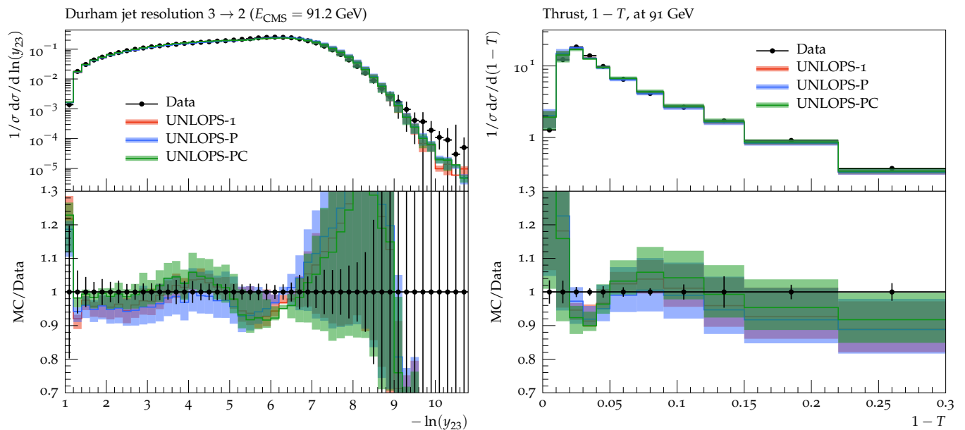
FIG. 2: Renormalization scale variation bands for the differential Durham jet resolution and thrust compared for the different variations of unitary NLO multi-jet merging. Data from [26] and [27].
