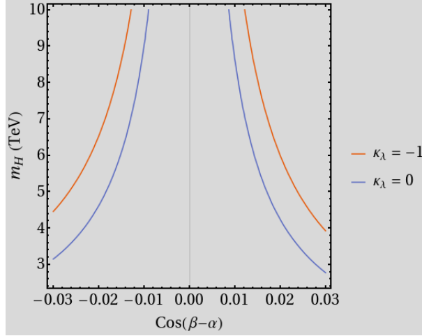
Figure 1: Contours of \kappa_\lambda in the \cos(\beta - \alpha) - m_H plane. In drawing this plot, we have assumed \sin 2\beta = 0.22 and m_h = 125 GeV.
