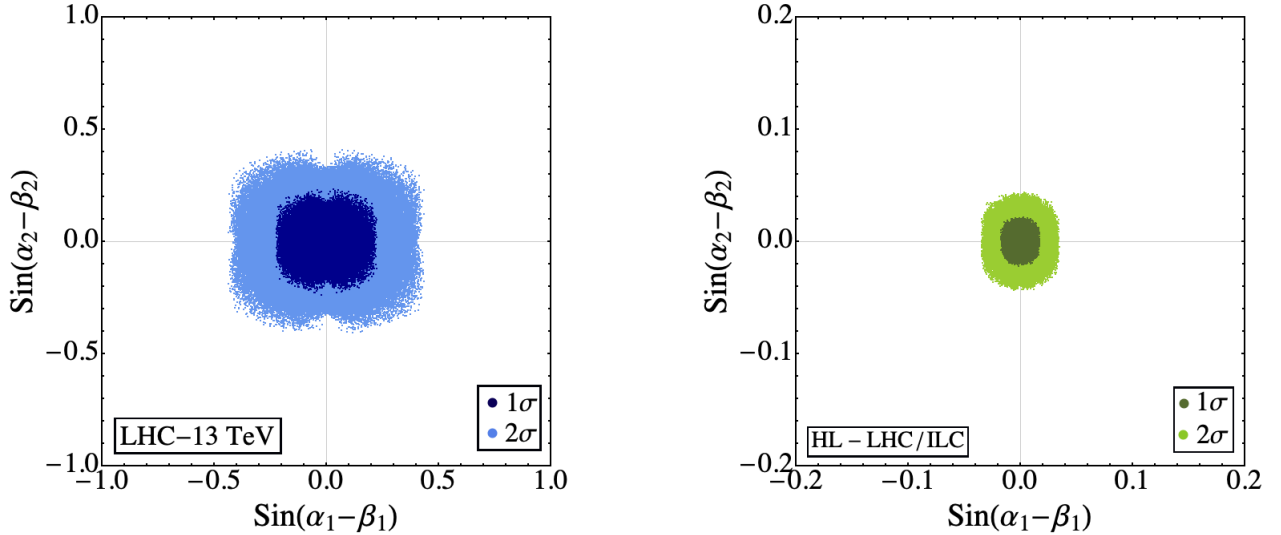
Figure 1: Allowed region in the \sin(\alpha_1 - \beta_1) - \sin(\alpha_2 - \beta_2) plane from the current (left panel) [2] and the future (right panel) [44] measurements of \kappa_x . The darker and lighter shades represent 1\sigma and 2\sigma allowed regions respectively. While extracting bound using the projected accuracies at the HL-LHC and the ILC, the central values for all the \kappa_x are assumed to be unity, i.e., consistent with the SM.
