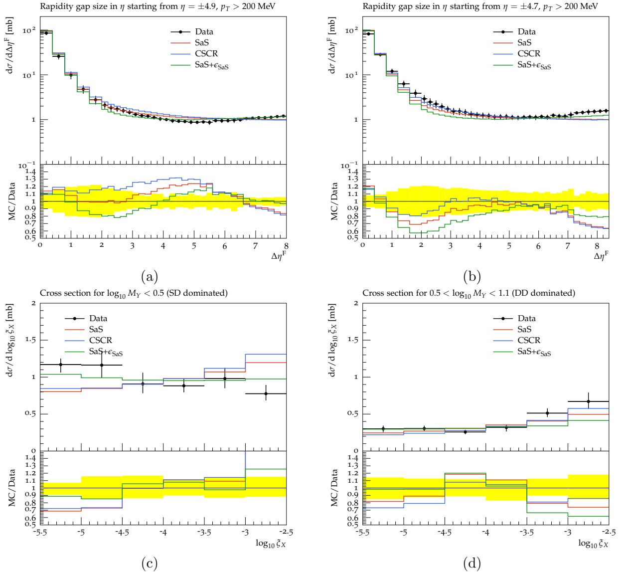
Figure 16: The cross section as a function of gap size for the three SaS-based models compared to ATLAS [52] (a) and CMS [53] (b) data. The cross section as a function of \log_{10} \xi_X in a single-diffractive dominated region (c) and double diffractive dominated region (d) compared to CMS [53] data.
