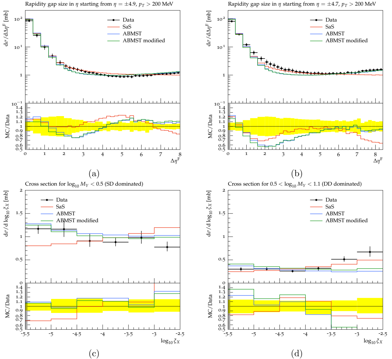
Figure 17: The cross section as a function of gap size for the two ABMST-based models compared to ATLAS [52] (a) and CMS [53] (b) data. The cross section as a function of \log_{10}\xi_X in a single-diffractive dominated region (c) and double diffractive dominated region (d) compared to CMS [53] data. For reference the tuned SaS model is also shown.
