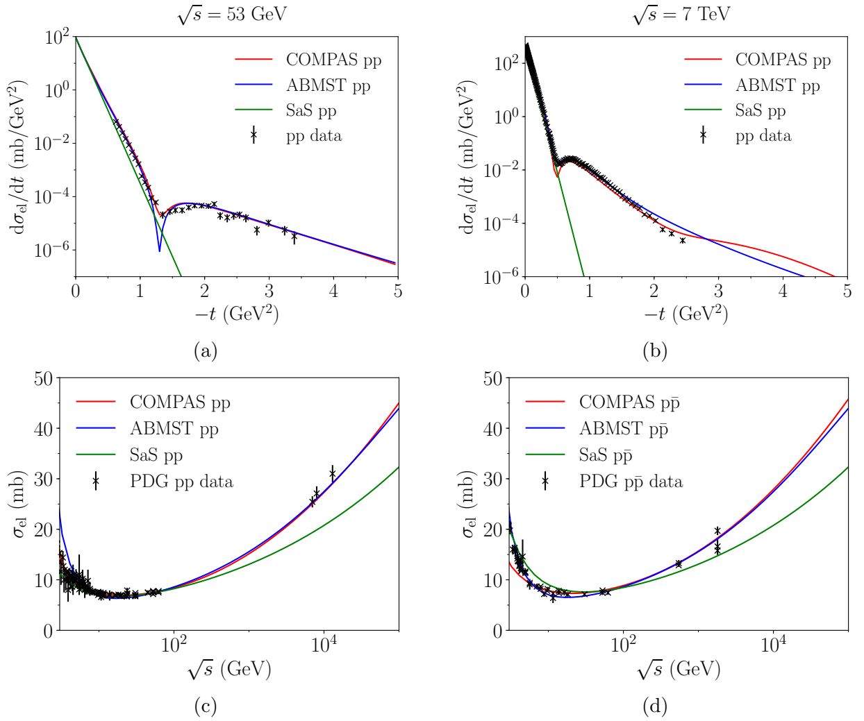
Figure 3: The elastic differential cross section parametrizations in \text{pp} collisions at 53 GeV (a) and 7 TeV (b). The integrated elastic cross section parametrizations in (c) \text{pp} and (d) \text{p}\bar{\text{p}} processes. Data from PDG [15].
