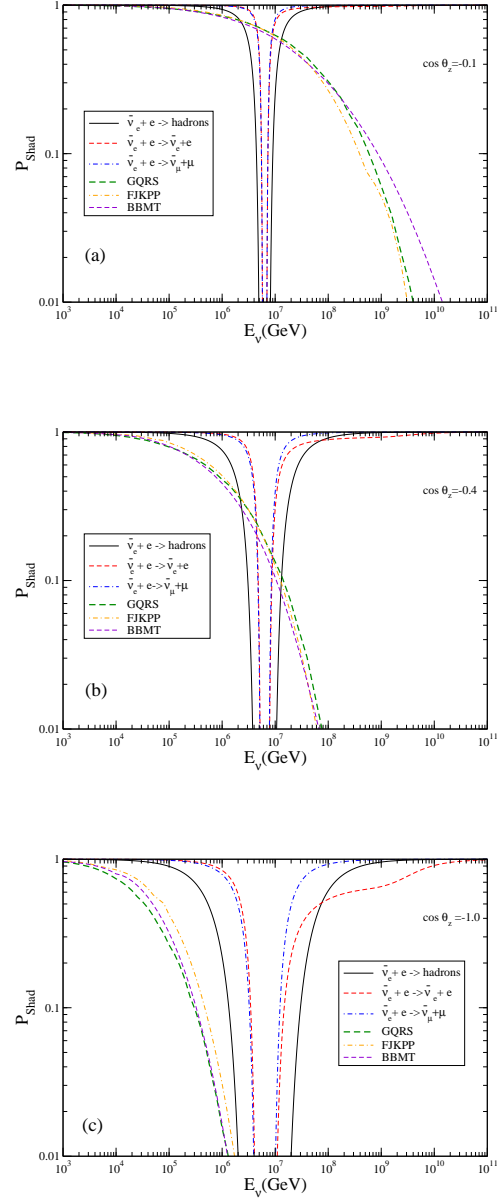
FIG. 2: (Color online) Energy dependence of the probability of neutrino absorption for different values of the angle of neutrino incidence.
