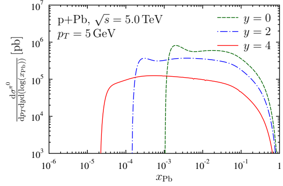
Figure 2: The contribution to differential cross section from different values of x_{Pb} for inclusive \pi^0 production in p+Pb collisions at \sqrt{s_{NN}} = 5.0 \text{ TeV} and p_T = 5 \text{ GeV/c} for \eta = 0 (dashed green), \eta = 2 (dot-dashed blue) and \eta = 4 (solid red). From Ref. [12].
