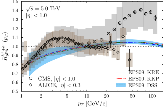
Figure 1: Nuclear modification factor for inclusive charged hadrons in p+Pb collisions at \sqrt{s_{NN}} = 5.0 \text{ TeV} . Data are from ALICE [7] (diamonds) and CMS [8] (circles) and the NLO pQCD results are calculated using CT10 PDFs with EPS09 nuclear modification and three FFs, see Ref. [10] for details.
