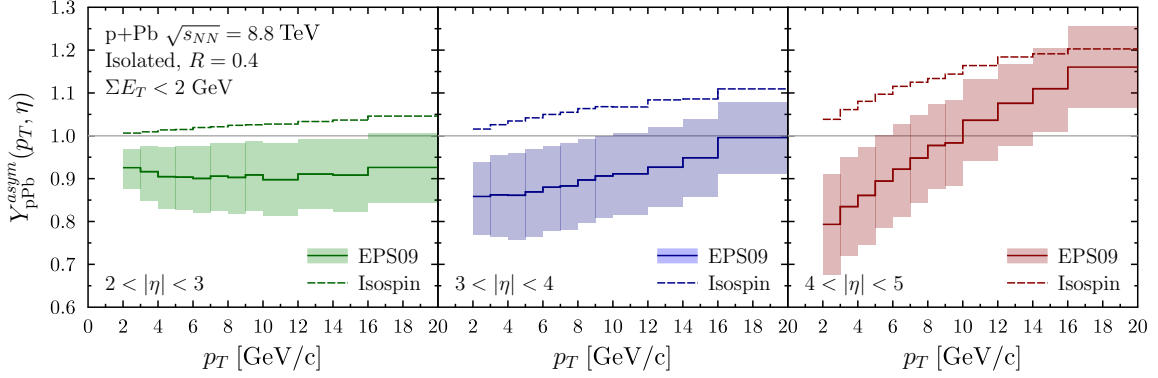
Figure 5: The yield asymmetry between forward and backward rapidities in p+Pb collisions at \sqrt{s_{\text{NN}}} = 8.8 TeV for three different rapidities, 2 < |\eta| < 3 (left), 3 < |\eta| < 4 (middle) and 4 < |\eta| < 5 (right). The isospin effect is plotted with dashed line to each panel. From Ref. [12].
