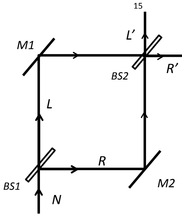
Figure 1. A simple Mach-Zehnder interferometer (MZI) setup, also exhibiting the notation used in the text. The beamsplitters are denoted BS1 , etc., the mirrors M1 , etc., and the arms L , R , etc.
