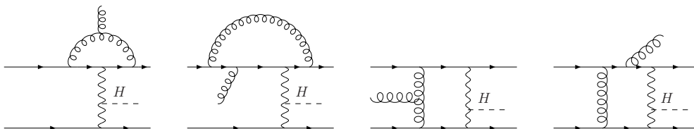
Figure 1: A subset of one-loop Feynman diagram topologies for EW Hjj production.
