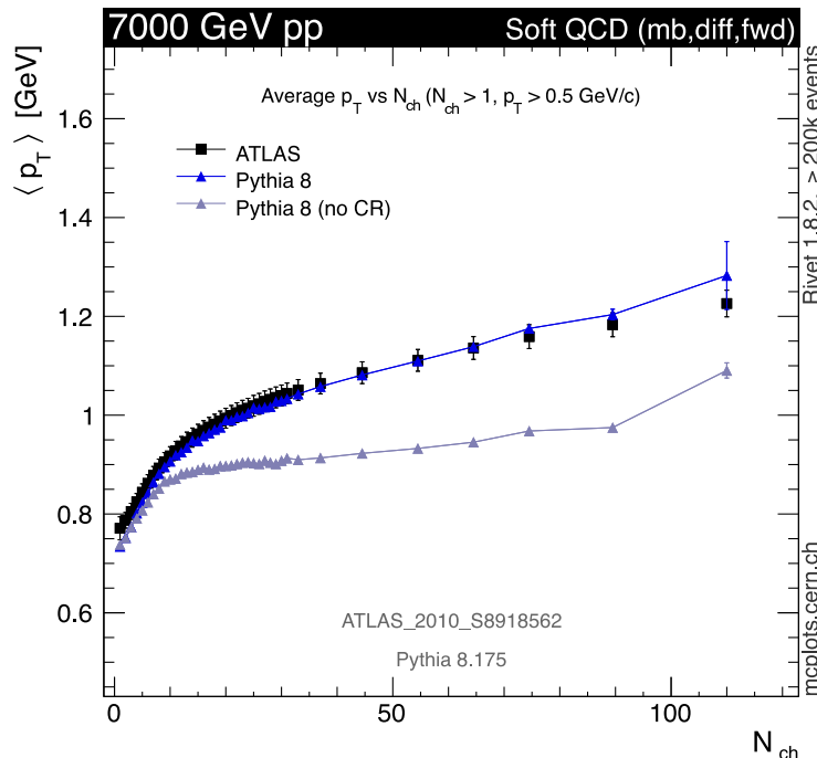
Figure 1: \langle p_{\perp} \rangle(n_{\text{ch}}) with the default PYTHIA 8 Tune 4C [21], and the same with CR switched off, compared with ATLAS data [22].
