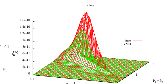
Fig. 9. The momentum distribution of the bare and the pure VMD pion-loop contribution for P_2 = P_1 .
