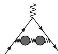
Fig. 4. A diagram with two insertions of the HVP.
