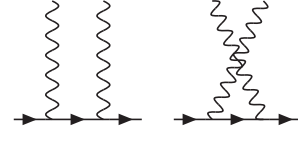
Fig. 7. The tree level diagrams that contract to the axial vector current in the limit P_1^2 \approx P_2^2 \gg Q^2 .
