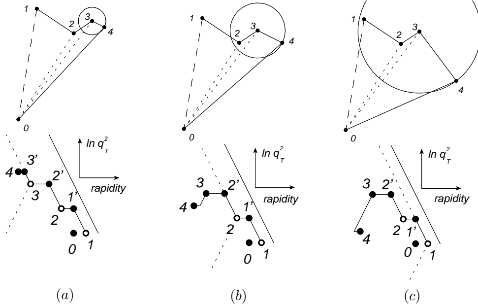
Figure 25: A parton emission (4), being emitted at different distances. The upper figures are in impact-parameter space, and the lower figures are in y - q_{\perp} representation, where the dotted lines show the limits of the q_{+} and q_{-} ordering. The circles in the upper figures show the coherence range of the emission.
