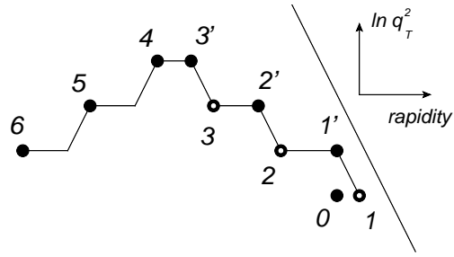
Figure 8: The same cascade as in fig. 8. The x direction shows rapidity, and y direction shows \ln(k_{\perp}^2) . The diagonal line is the constant p_+ of the incoming particle.
