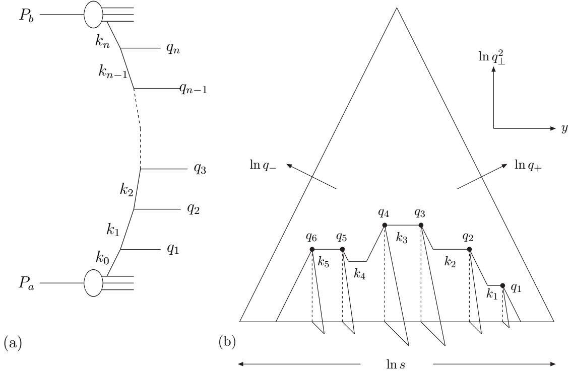
Figure 5: (a) A parton chain stretched between projectile and target. (b) A backbone of k_\perp -changing gluons in a (y, \ln q_\perp^2) plane. The transverse momentum of the virtual links k_i are represented by horizontal lines.
